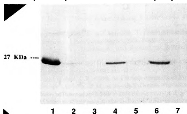
Fig. 2. Western blot analysis of Drosophila ADH. Control ADH, purified from D. melanogaster flies, was loaded in lanes (1) 0.05 mg. and (2) 1 µg. Protein extracts were from the following yeast strains (3) 20 µl of Y-φ (WV201-36 transformed with pVT-U plasmid without insert), (4) 20 µl of Y-Phe (WV201-36 transformed with pVT-Adh-Phe 152 mutant plasmid), and (6) 5 µl of Y-Wt (WV201-36 transformed with pVT-Adh wild-type plasmid). (5) and (7) are plain sample buffer.
